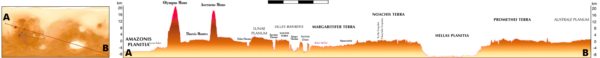
Cross section of Mars, through Olympus Mons and Hellas Planitia
